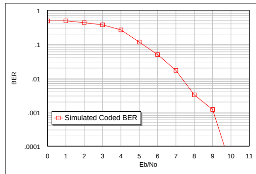
16QAM
