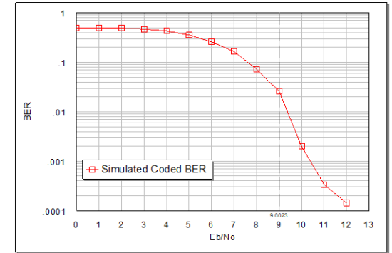
16PSK
