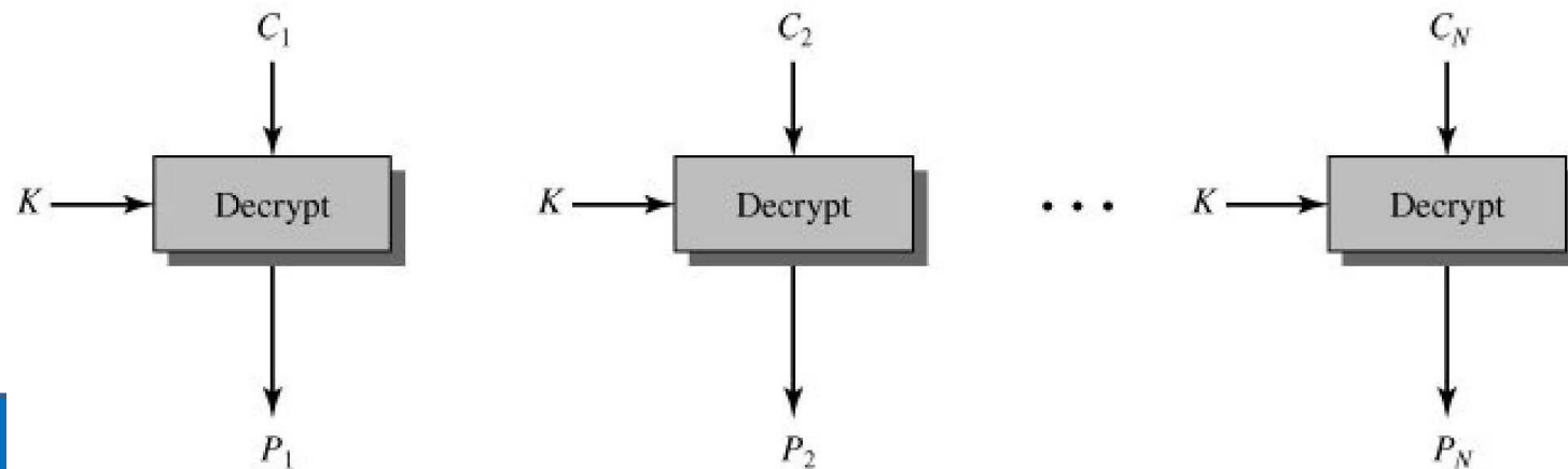
(b) Decryption
