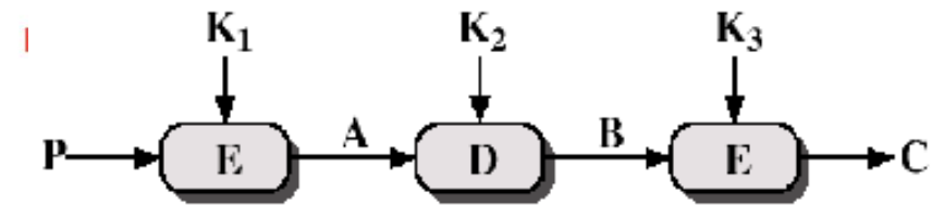
(a) Encryption
