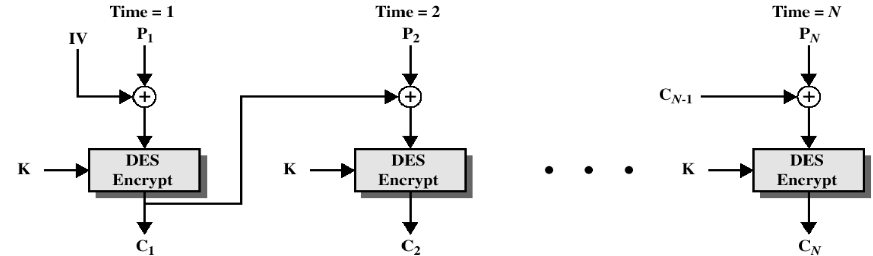
(a) Encryption
