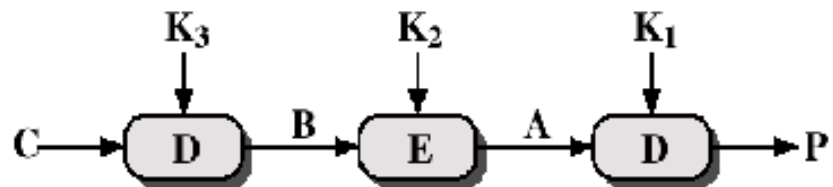
(b) Decryption
