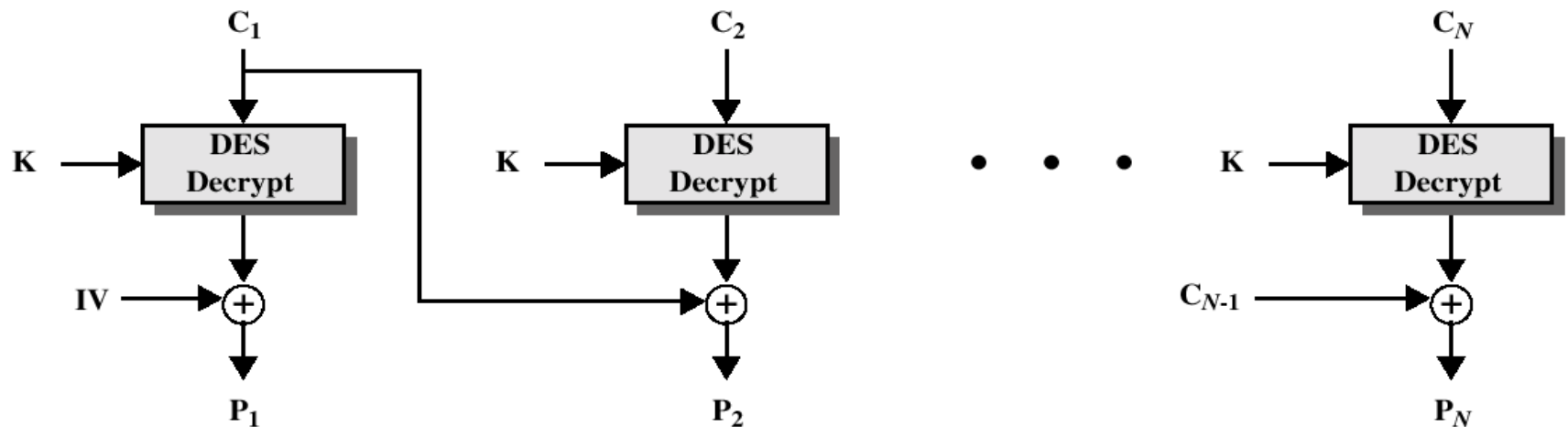
(b) Decryption
