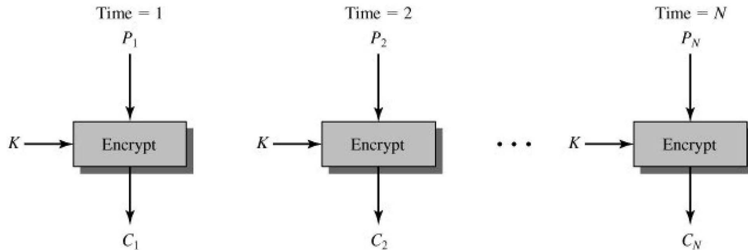
(a) Encryption
