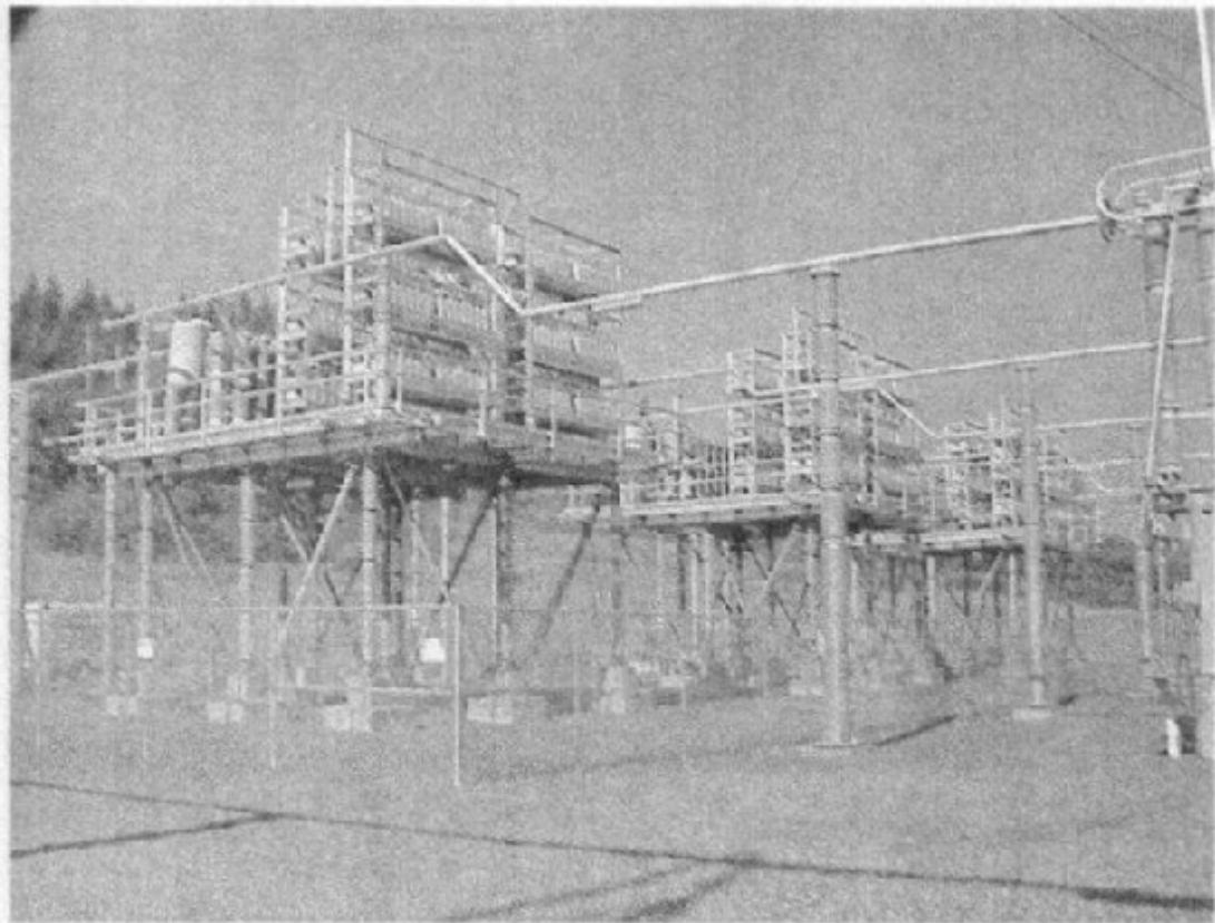
Series Capacitor.
