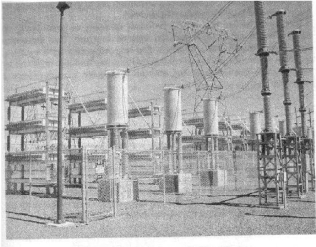
Current-Limiting Inductor or Air Core Reactor.
