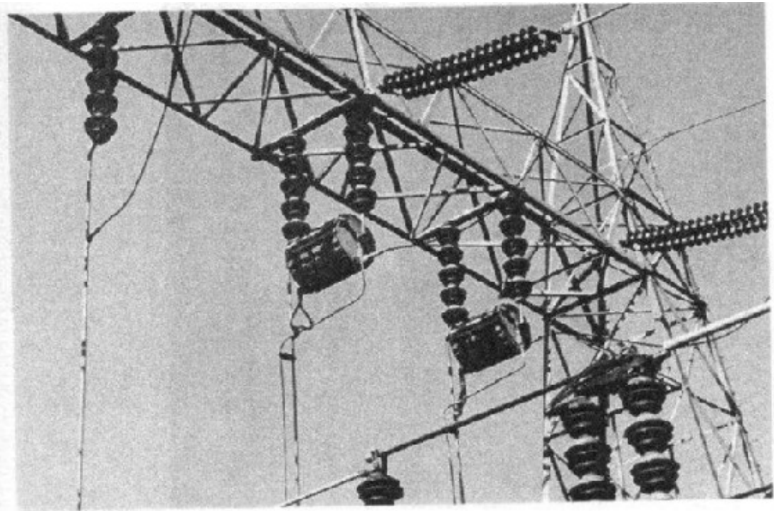
Line Trap.
