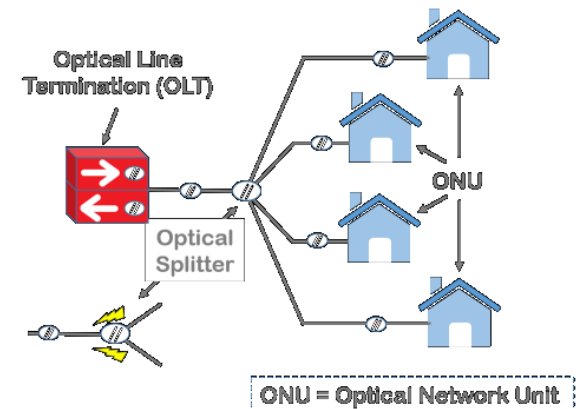
Passive Optical Network | PON
