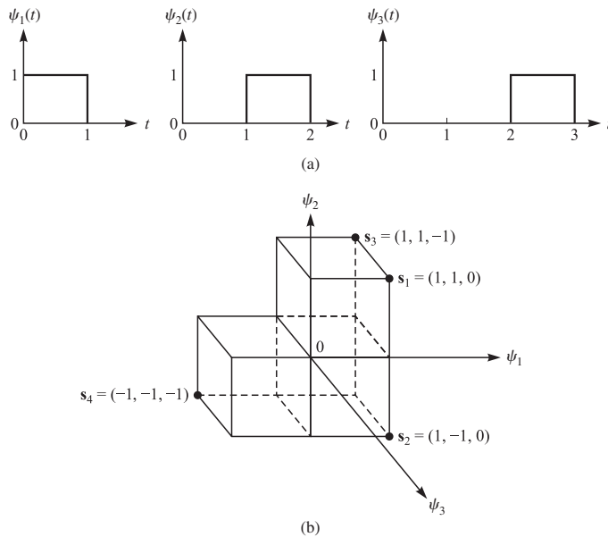
FIGURE 2.2-4 An alternative set of orthonormal functions for the four signals in Figure 2.2-1(a) and the corresponding signal points.
