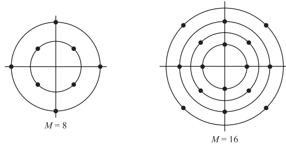
FIGURE 3.2-4 Examples of combined PAM-PSK constellations.
