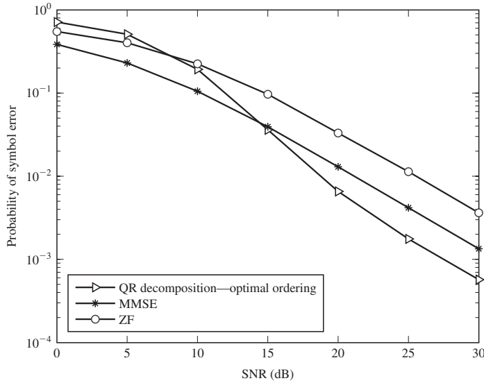
FIGURE 16.4-8 Comparison of the QR decomposition and the linear precoders with N_T = K = 4 .
