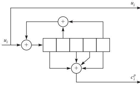
FIGURE 8.9–2 A (31, 27) RSC encoder.
