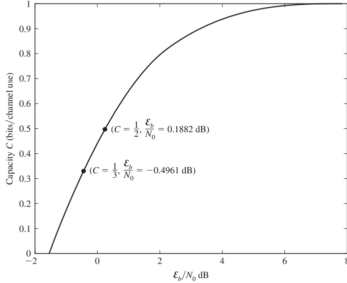
FIGURE 6.5-6 The capacity of binary input AWGN channel.
