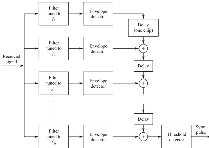
FIGURE 12.5–2 System for acquisition of an FH signal.
