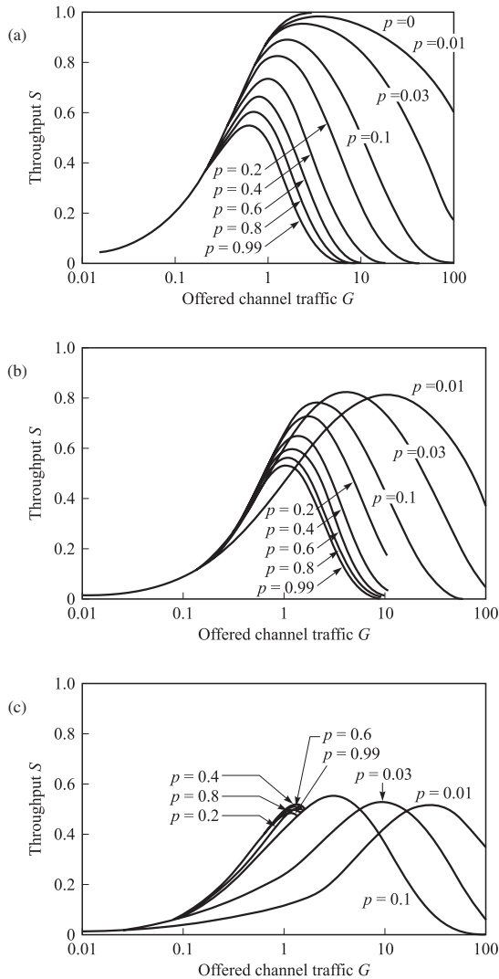
FIGURE 16.5-6 Channel throughput in p -persistent CSMA: (a) a = 0 ; (b) a = 0.01 ; (c) a = 0.1 . [From Kleinrock and Tobagi (1975), © IEEE.]
