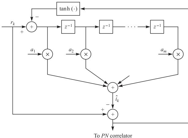
FIGURE 12.2-18 Non-linear excision filter.
