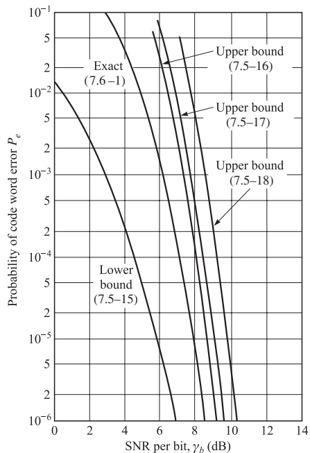
FIGURE 7.6-1 Comparison of bounds with exact error probability for hard decision decoding of Golay (23, 12) code.
