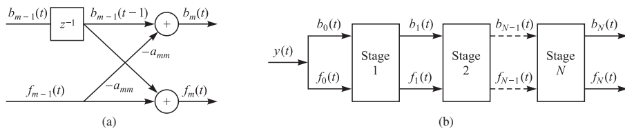
FIGURE 10.4-2 A lattice filter.
