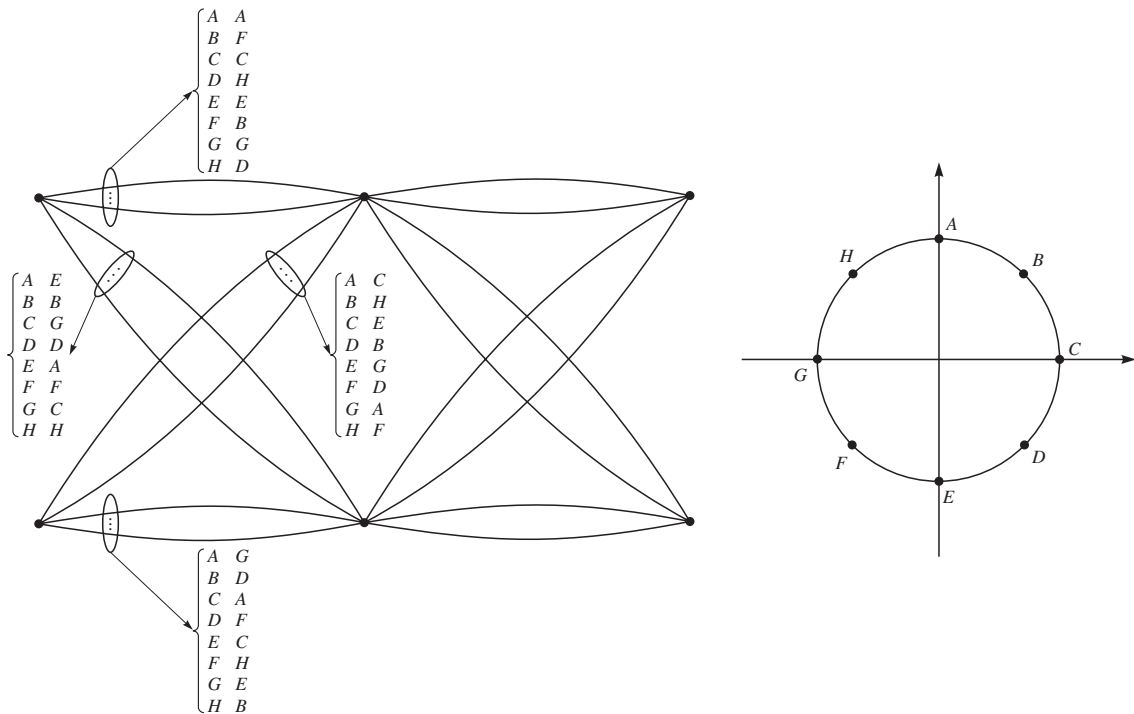
FIGURE 14.5-4 An example of multiple trellis-coded modulation.
