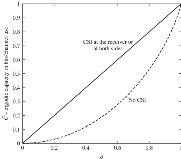
FIGURE 14.2–2 The ergodic capacity of channel model 1.
