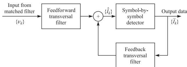
FIGURE 9.5–1 Structure of decision-feedback equalizer.
