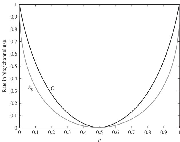
FIGURE 6.8-1 Cutoff rate and channel capacity plots for a binary symmetric channel.
