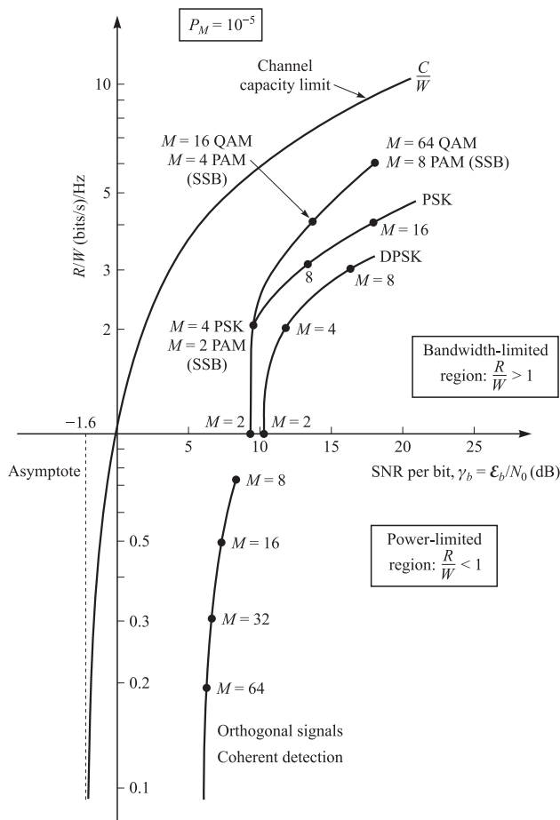
FIGURE 4.6–1 Comparison of several modulation schemes at P_e = 10^{-5} symbol error probability.
