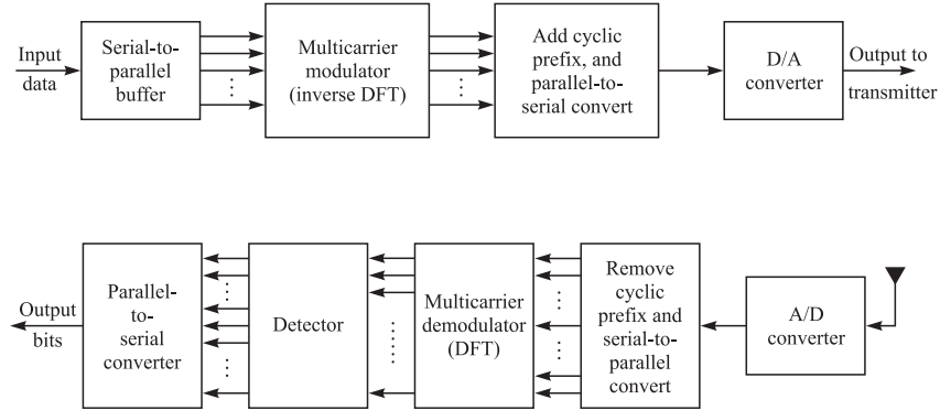
FIGURE 11.2-4 Multicarrier communication system.
