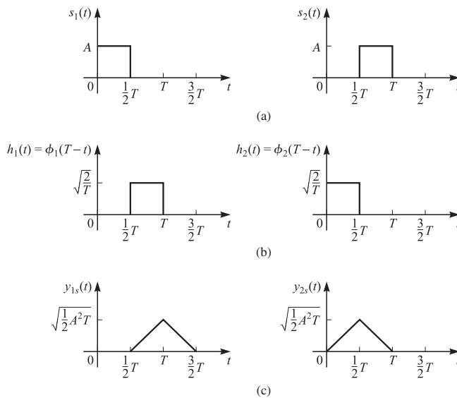
FIGURE 4.2-9 Basis functions and matched filter response for Example 4.2–1.
