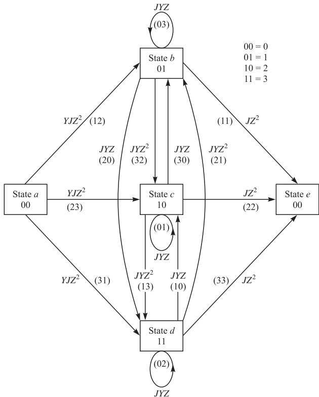
FIGURE 8.1-14 State diagram for K = 2, k = 2 , rate 1/2 nonbinary code.
