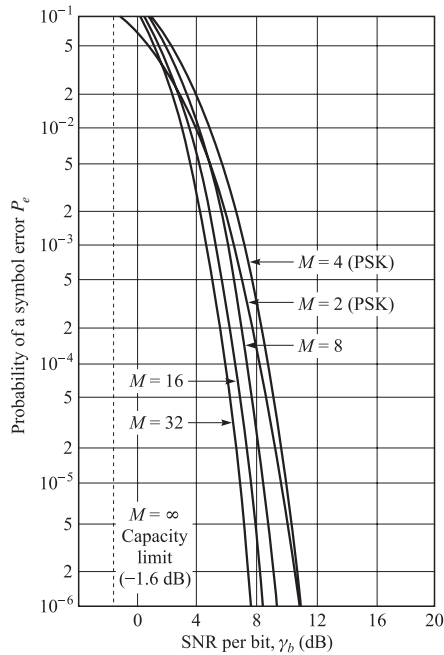
FIGURE 4.4-2 Probability of symbol error for biorthogonal signals.
