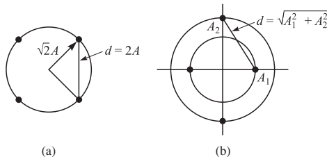
FIGURE 4.3-6 Two four-point signal constellations.
