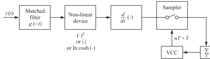
FIGURE 5.3–2 Non-decision-directed estimation of timing for binary baseband PAM.
