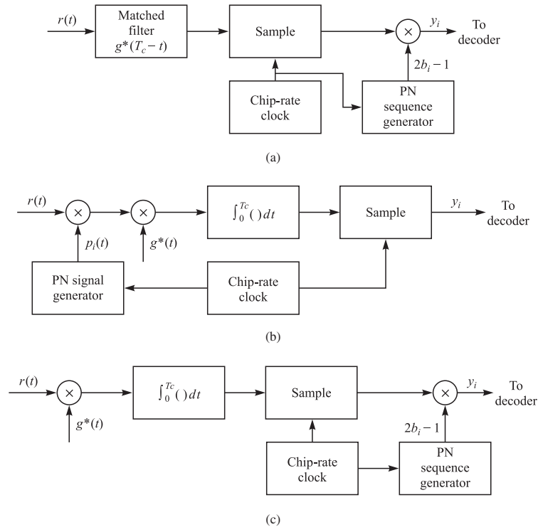
FIGURE 12.2-2 Possible demodulator structures for PN spread spectrum signals.
