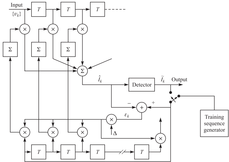
FIGURE 10.1-1 An adaptive zero-forcing equalizer.
