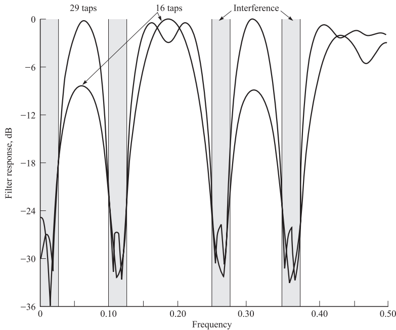
FIGURE 12.2–16 Frequency-response characteristics of 16- and 29-tap filters for four bands of interference.
