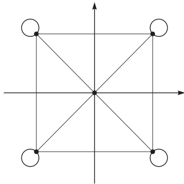
FIGURE 3.3-12 The in-phase and quadrature components for QPSK.
