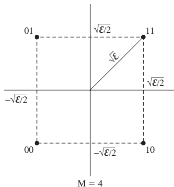
FIGURE 3.3-11 A possible mapping for QPSK signal.
