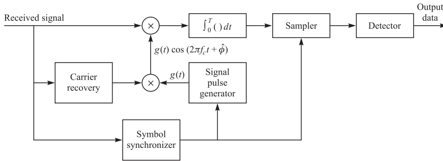
FIGURE 5.1-1 Block diagram of a binary PSK receiver.
