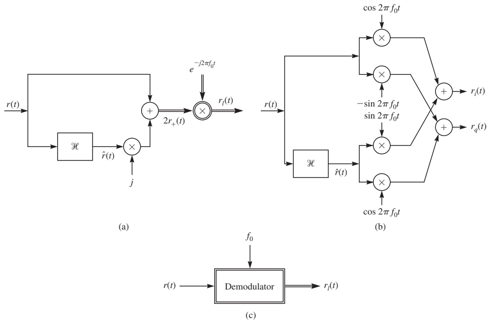
FIGURE 4.3–9 Complex (a) and real (b) demodulators. A general representation for a demodulator is shown in (c).
