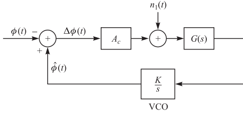
FIGURE 5.2–7 Linearized PLL model with additive noise.
