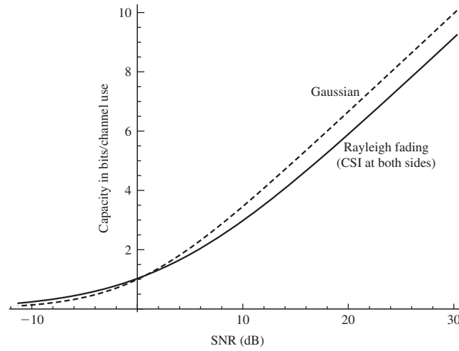
FIGURE 14.2-5 Capacity of Gaussian and Rayleigh fading channel with CSI at both sides.
