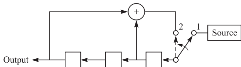
FIGURE 7.9-8 Three-stage ( m = 3 ) shift register with feedback.
