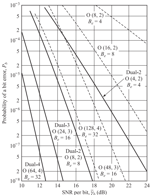
FIGURE 14.7-7 Comparison of performance between block orthogonal codes and dual- k with block orthogonal inner codes.
