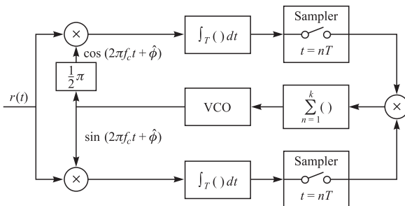
FIGURE 5.2–13 Non-decision-directed PLL for carrier phase estimation of PAM signals.
