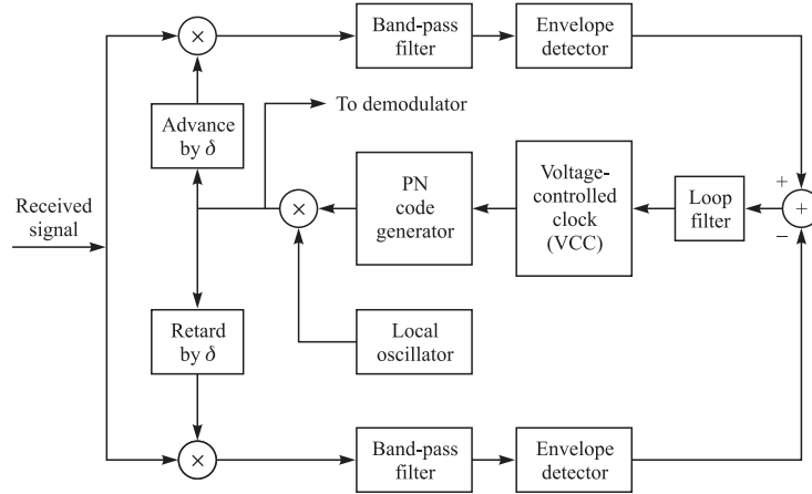
FIGURE 12.5-5 Delay-locked loop (DLL) for PN code tracking.
