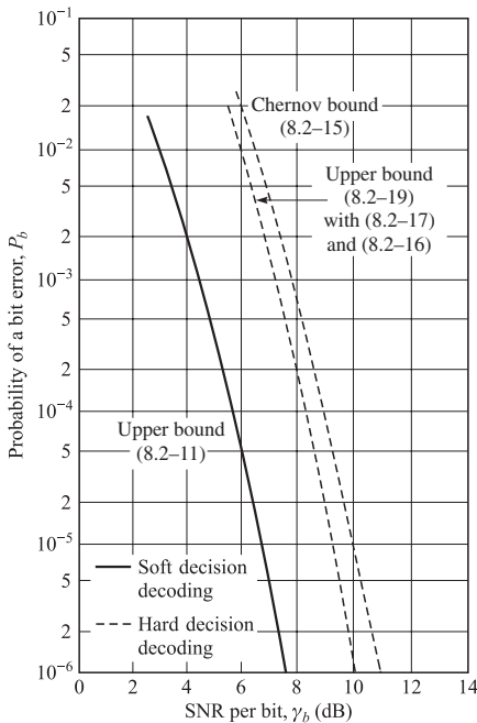
FIGURE 8.2-1 Comparison of soft decision and hard decision decoding for K = 3, k = 1, n = 3 convolutional code.
