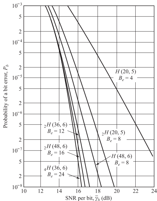
FIGURE 14.7-5 Performance of Hadamard codes.
