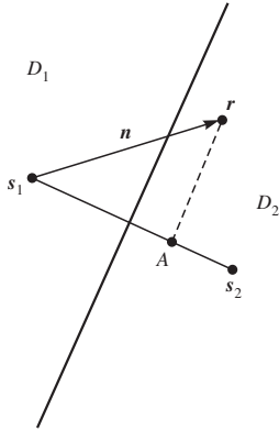
FIGURE 4.2-3 Decision regions for binary equiprobable signals.
