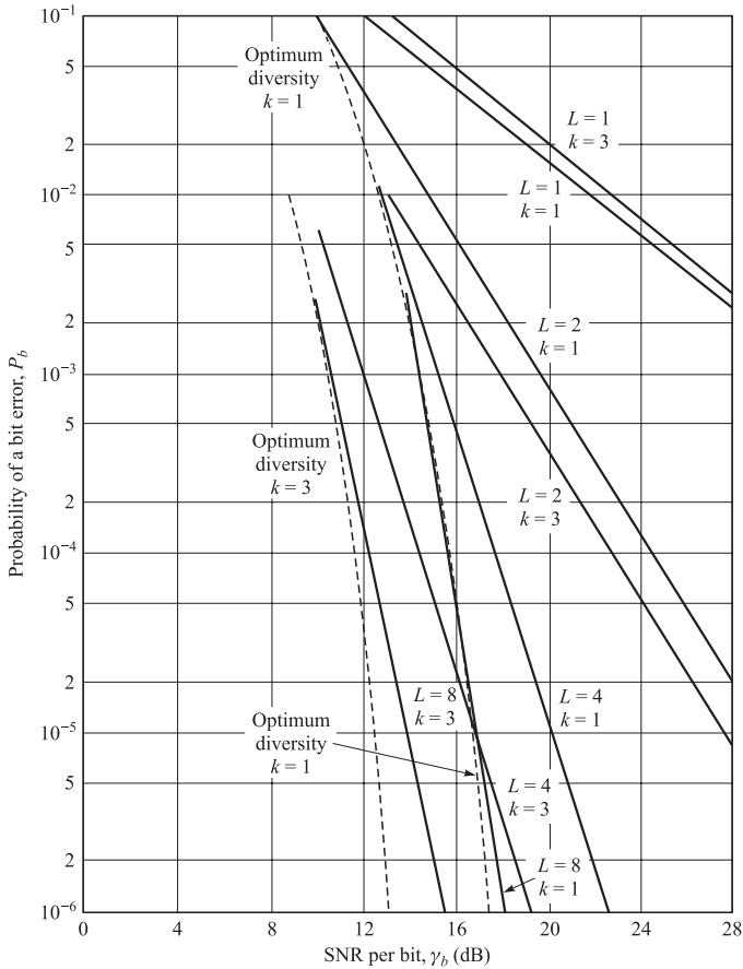
FIGURE 12.3-6 Performance of binary and octal FSK with L -order diversity for a channel with worst-case partial-band interference.
