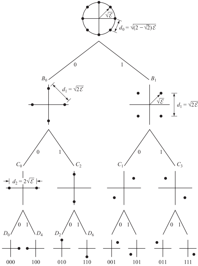
FIGURE 8.12-1 Set partitioning of an 8-PSK signal set.
