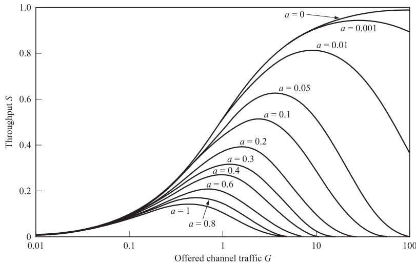
FIGURE 16.5-5 Throughput in nonpersistent CSMA. [From Kleinrock and Tobagi (1975), © IEEE.]
