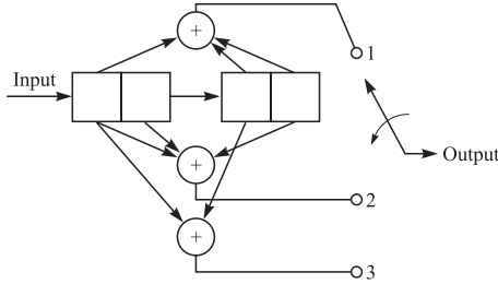
FIGURE 8.1-3 K = 2, k = 2, n = 3 convolutional encoder.
