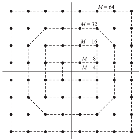
FIGURE 4.7-2 QAM constellation.
