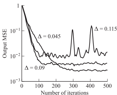
FIGURE 10.1-4 Initial convergence characteristics of the LMS algorithm with different step sizes. (From Digital Signal Processing , by J. G. Proakis and D. G. Manolakis, 1995, Prentice Hall Company. Reprinted with permission of the publisher.)
