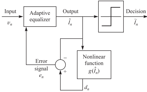
FIGURE 10.5–1 Adaptive blind equalization with stochastic gradient algorithms.
