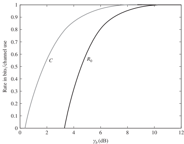
FIGURE 6.8-2 Capacity and cutoff rate for an output quantized BPSK scheme.
