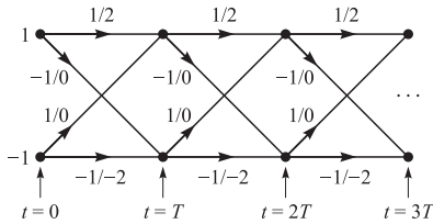
FIGURE 9.2-12 Trellis for duobinary partial-response signal.
