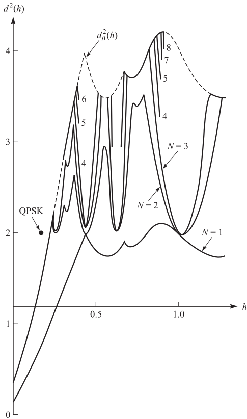
FIGURE 4.9-7 Squared minimum Euclidean distance as a function of the modulation index for quaternary CPFSK. The upper bound is d_B^2 . [From Aulin and Sundberg (1981), © 1981 IEEE.]
