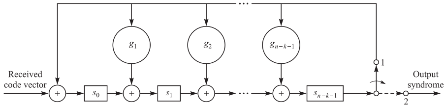
FIGURE 7.9-6 An (n - k) -stage shift register for computing the syndrome.
