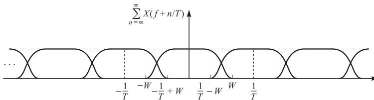
FIGURE 9.2-6 Plot of B(f) for the case T > 1/2W .
