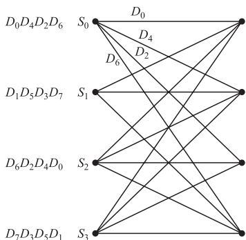
FIGURE 8.12–7 An alternative four-state trellis code.
