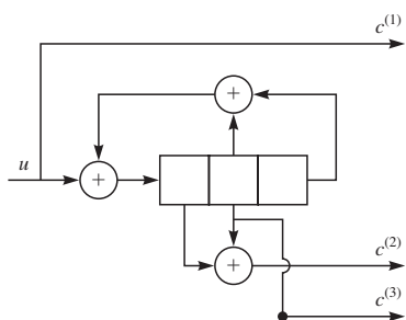
FIGURE 8.1-16 Realization of G'(D) using feedback shift register.
