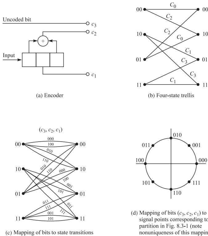
FIGURE 8.12-4 Four-state trellis-coded modulation with 8-PSK signal constellation.
