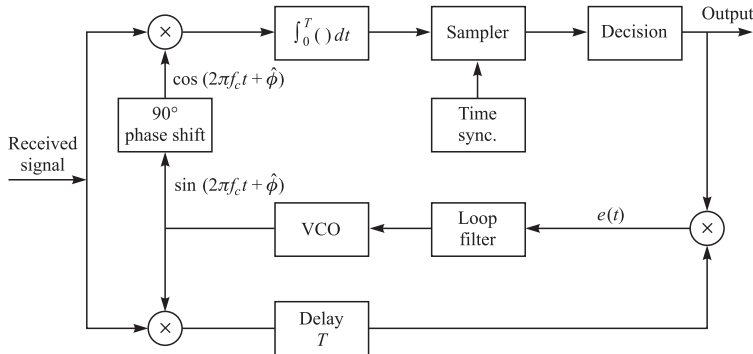
FIGURE 5.2-10 Carrier recovery with a decision-feedback PLL.
