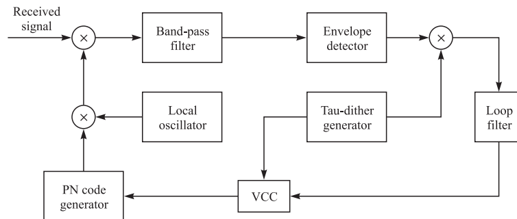
FIGURE 12.5-6 Tau-dither loop (TDL).
