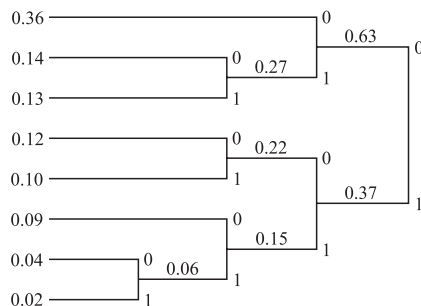
FIGURE 6.3-6 Huffman code for Example 6.3-2.
