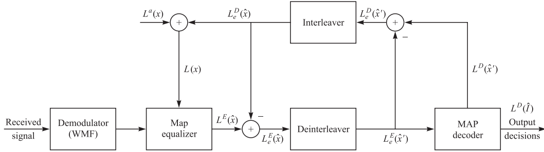
FIGURE 9.7-1 Iterative equalization and decoding.
