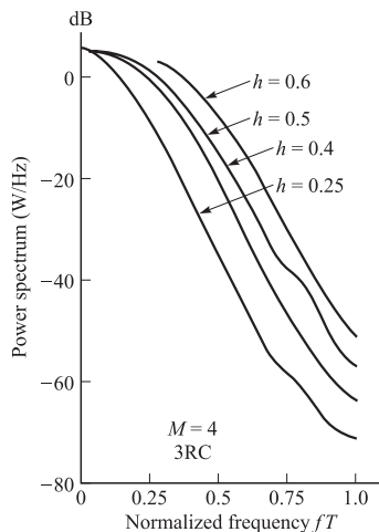
FIGURE 3.4-7 Power spectral density for M = 4 CPM with 3RC and different modulation indices. [Source: Aulin et al. (1981); © IEEE.]
