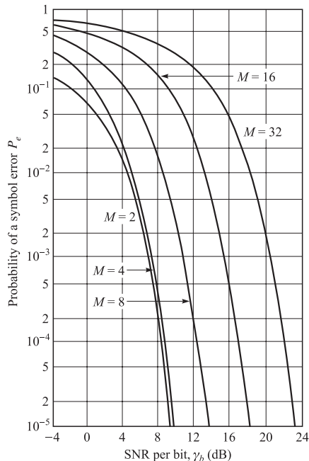
FIGURE 4.3–5 Probability of symbol error for PSK signals.
