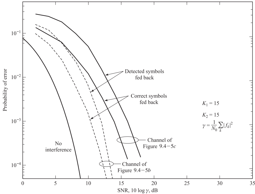
FIGURE 9.5-2 Performance of decision-feedback equalizer with and without error propagation.
