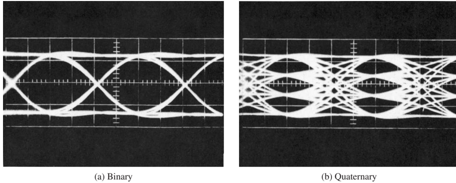
FIGURE 9.2-1 Examples of eye patterns for binary and quaternary amplitude-shift keying (or PAM).
