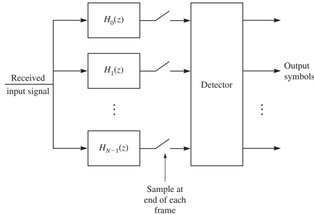
FIGURE 11.2–7 Filter bank implementation of OFDM receiver.
