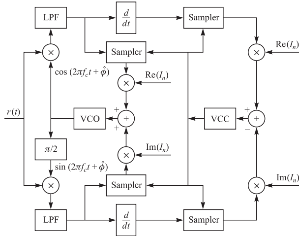
FIGURE 5.4-1 Decision-directed joint tracking loop for carrier phase and symbol timing in QAM and PSK.
