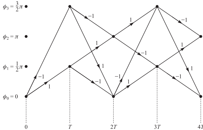
FIGURE 3.3-9 State trellis for binary CPFSK with h = \frac{1}{2} .
