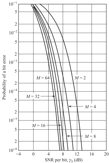
FIGURE 4.4-1 Probability of bit error for orthogonal signaling.
