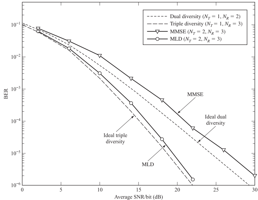
FIGURE 15.1-4 Performance of MLD and MMSE detectors with N_R = 3 receiving antennas.
