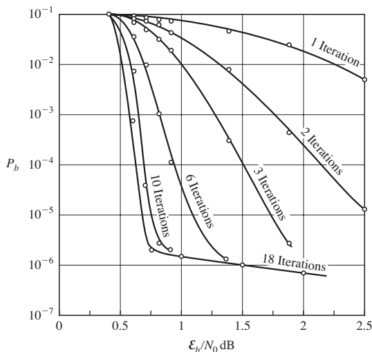
FIGURE 8.9-4 Performance of iterative decoding for turbo codes.
