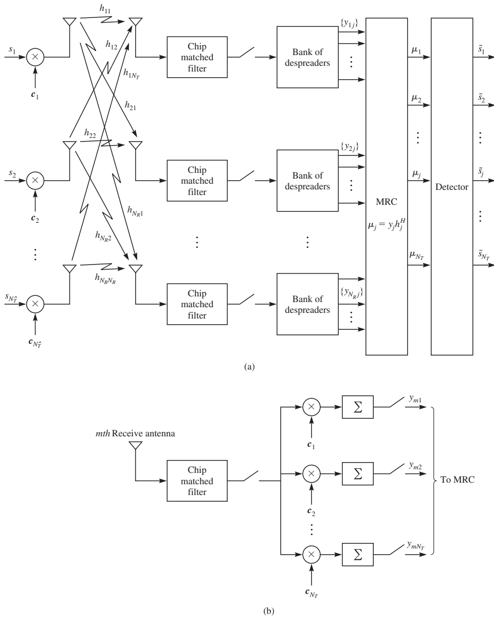
FIGURE 15.3-1 MIMO system with spread spectrum signals.
