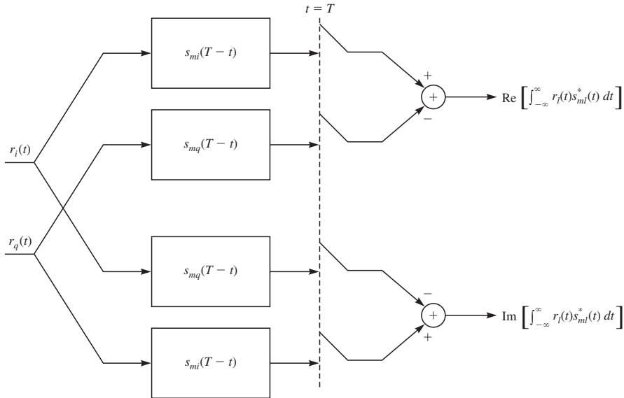
FIGURE 4.3–11 Equivalent lowpass matched filter.
