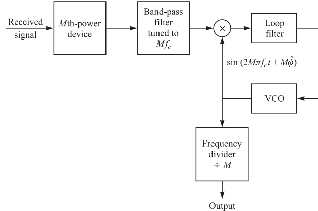
FIGURE 5.2–16 Carrier recovery with M th-power-law device for M -ary PSK.
