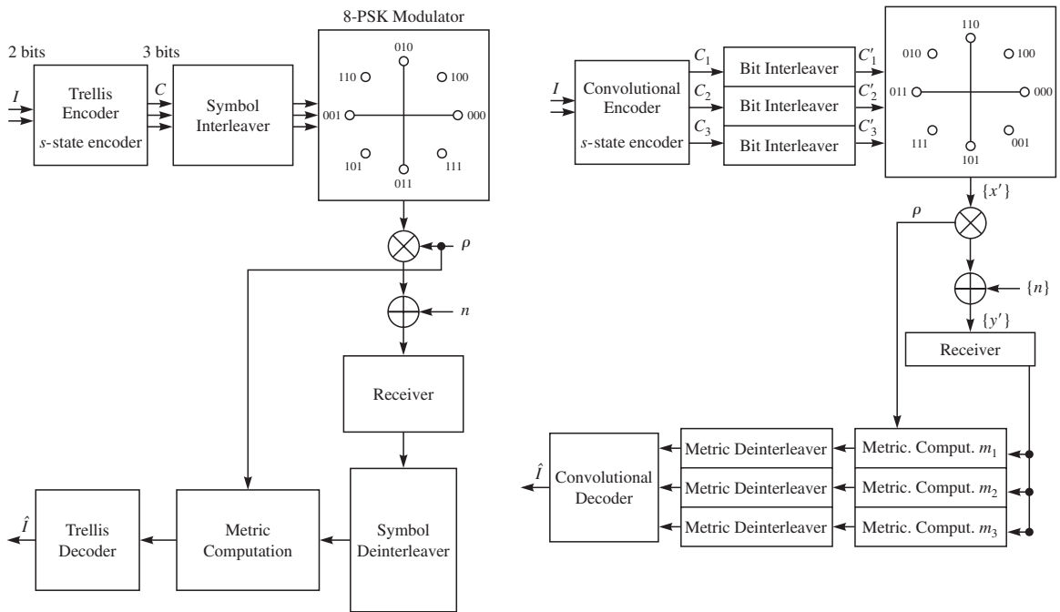
FIGURE 14.6–1 A TCM system (left) and a BICM system (right). [From Zehavi (1992) copyright IEEE.]
