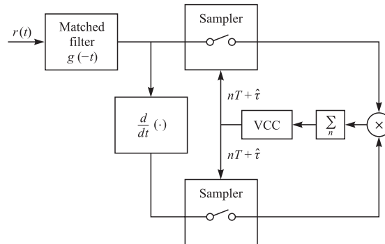
FIGURE 5.3–3 Non-decision-directed estimation of timing for baseband PAM.
