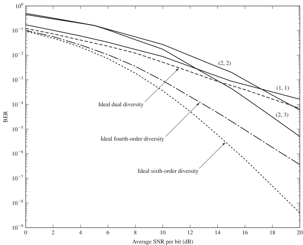
FIGURE 15.1-9 Performance of DFEs for two-path channel with (N_T, N_R) antennas for spatial multiplexing.
