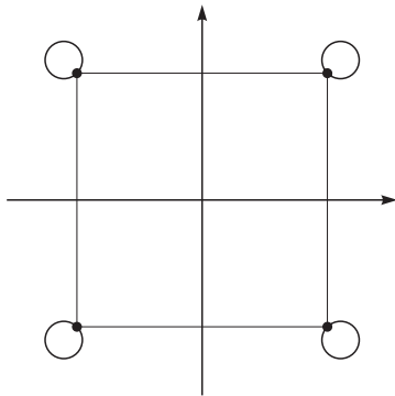
FIGURE 3.3-14 The in-phase and quadrature components for OQPSK signaling.
