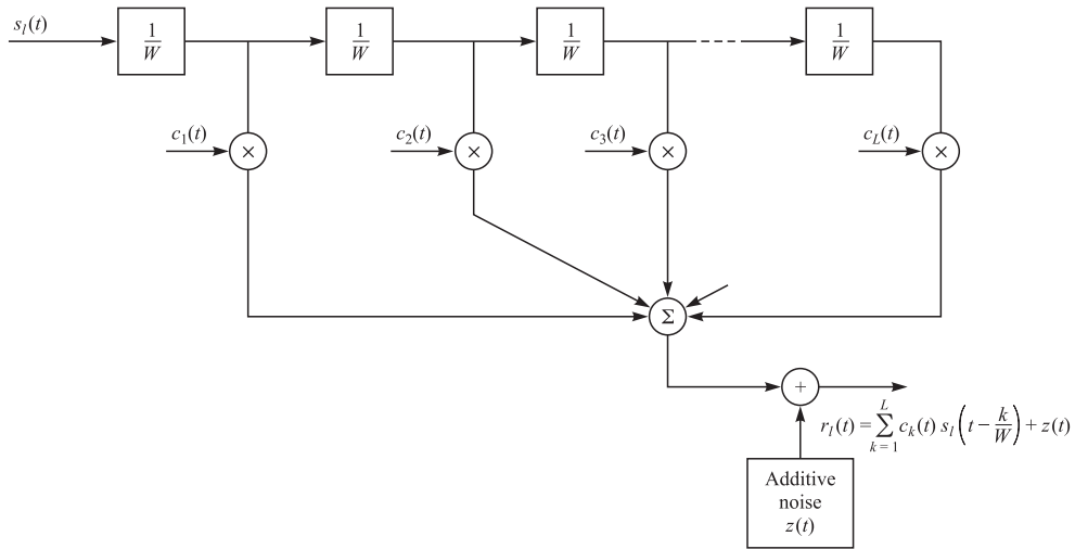
FIGURE 13.5-1 Trapped delay line model of frequency-selective channel.
