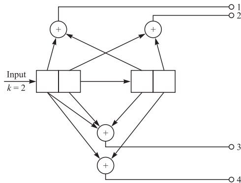
FIGURE 8.1-11 K = 2, k = 2, n = 4 convolutional encoder.
