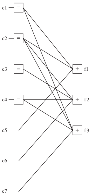
FIGURE 8.10-7 The factor graph representation for a (7, 4) Hamming code.
