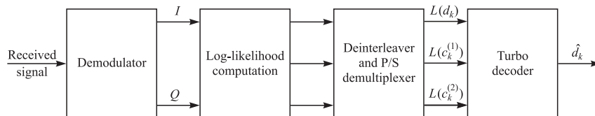
FIGURE 8.12–15 Decoder for concatenated PCCC/TCM code.
