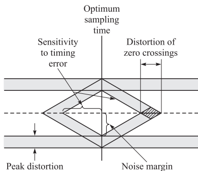
FIGURE 9.2-2 Effect of intersymbol interference on eye opening.
