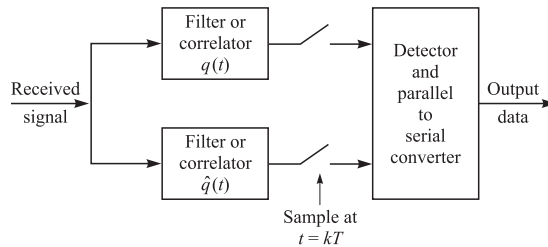
(b) Demodulator
