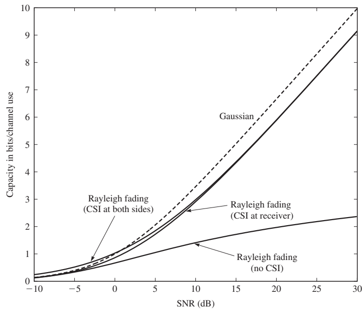
FIGURE 14.2-6 Capacity of Gaussian and Rayleigh fading channel with different CSI.
