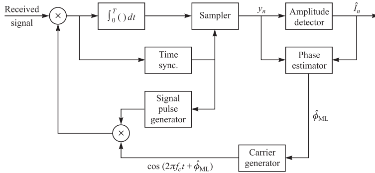
FIGURE 5.2-9 Block diagram of double-sideband PAM signal receiver with decision-directed carrier phase estimation.
