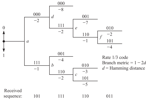
FIGURE 8.5-3 An example of the stack algorithm for decoding a rate 1/3 convolutional code.
