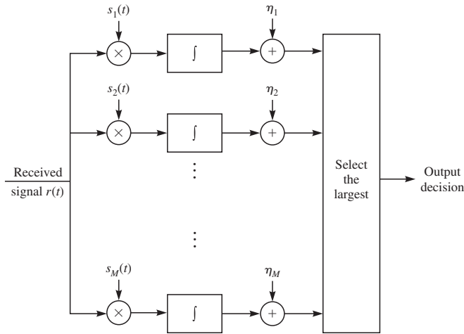
FIGURE 4.2–7 The structure of the correlation receiver with M correlators.
