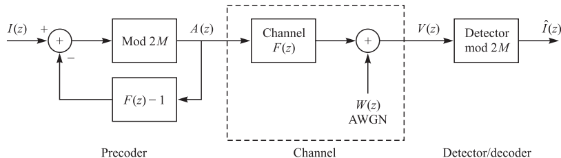
FIGURE 9.5–5 Tomlinson–Harashima precoding.
