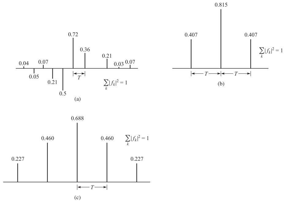
FIGURE 9.4-5 Three discrete-time channel characteristics.
