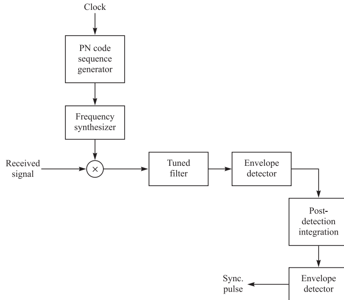
FIGURE 12.5-3 Alternative system for acquisition of an FH signal.
