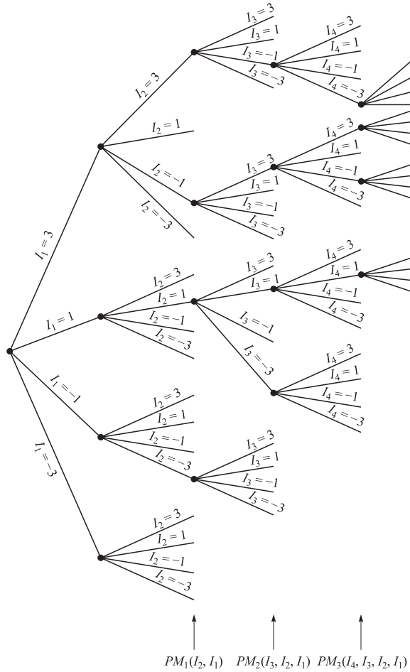
FIGURE 9.3-5 Tree diagram for Viterbi decoding of the duobinary pulse.
