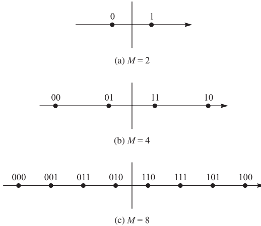
FIGURE 3.2-1 Constellation for PAM signaling.
