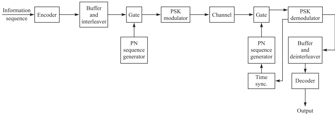
FIGURE 12.4-1 Block diagram of time-hopping (TH) spread spectrum system.
