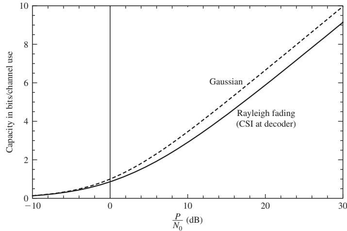
FIGURE 14.2-4 Capacity of Gaussian and Rayleigh fading channel with CSI at the decoder.
