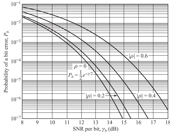
FIGURE 4.5-3 Probability of error for noncoherent detection of binary FSK.
