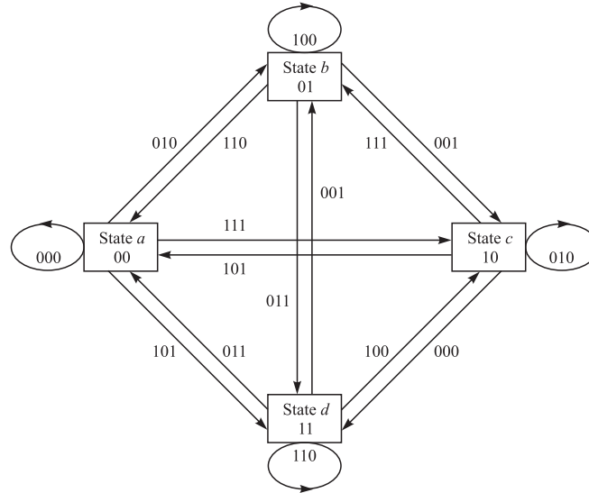
FIGURE 8.1-10 State diagram for K = 2, k = 2, n = 3 convolutional code.
