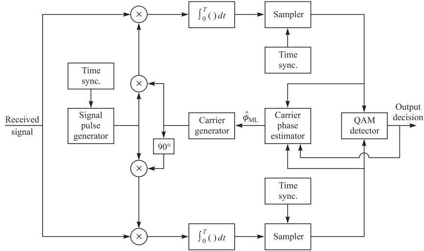
FIGURE 5.2–11 Block diagram of QAM signal receiver with decision-directed carrier phase estimation.
