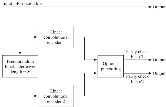
FIGURE 8.9-1 Encoder for parallel concatenated code (turbo code).
