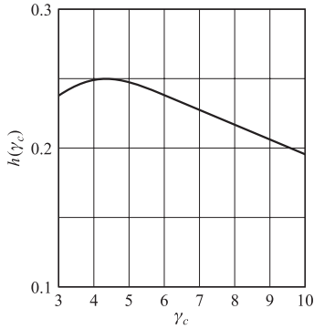
FIGURE 12.3-5 Graph of the function h(\gamma_c) .
