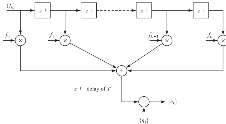
FIGURE 9.3-3 Equivalent discrete-time model of intersymbol interference channel with AWGN.
