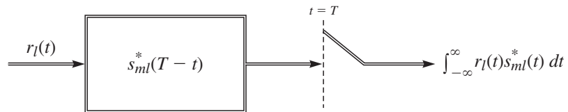
FIGURE 4.3–10 Complex lowpass equivalent matched filter.
