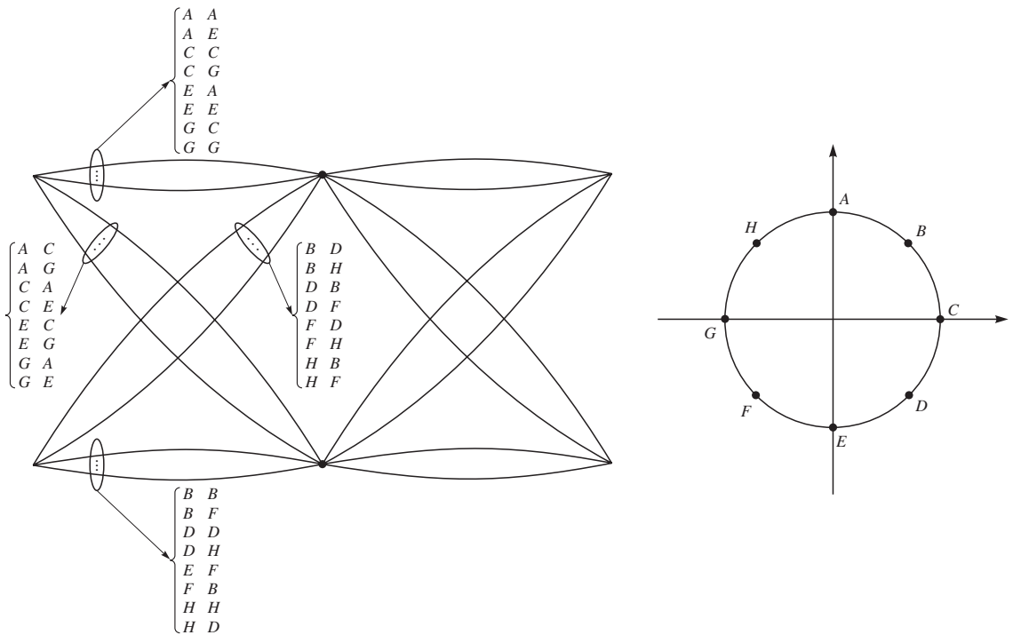
FIGURE 14.5-5 Signal assignment for an MTCM scheme appropriate for transmission over an AWGN channel.
