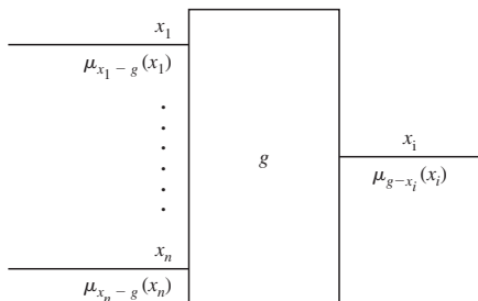
FIGURE 8.10-9 The local computation in sum-product algorithm.
