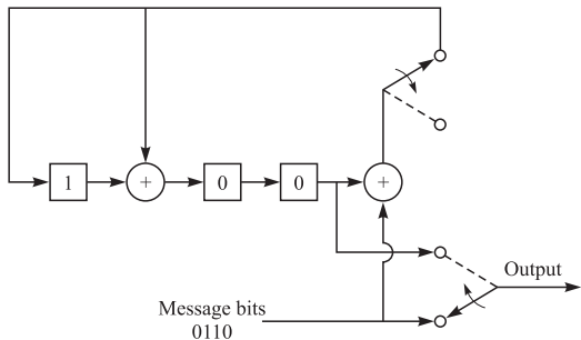
FIGURE 7.9-3 The encoder for the (7, 4) cyclic code with generator polynomial g(X) = X^3 + X + 1 .
