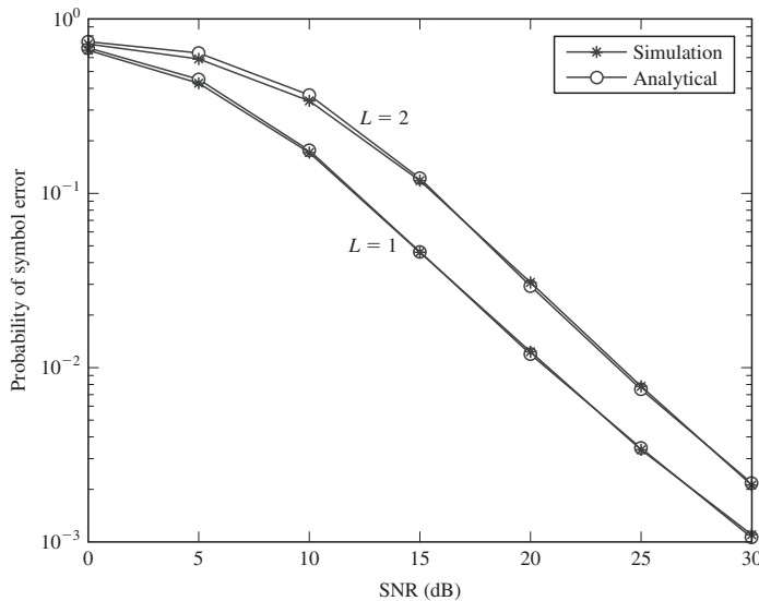
FIGURE 16.4-6 Performance of optimal QR decomposition with N_T = K = 2 and L = 1 and 2.
