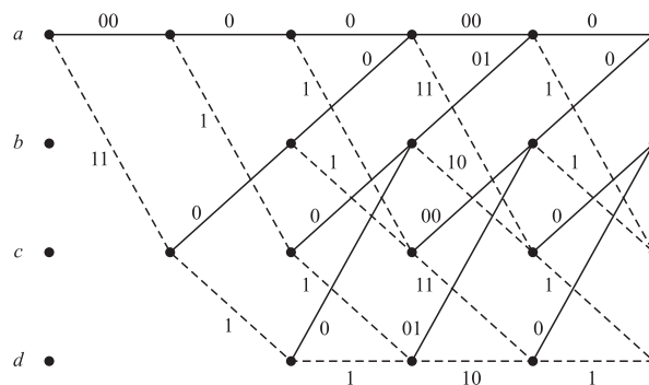
(b) Trellis of punctured code
