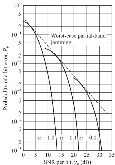
FIGURE 12.3-4 Performance of binary FSK with partial-band interference.
