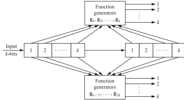
FIGURE 8.7-1 Encoder for rate 1/2 dual- k codes.
