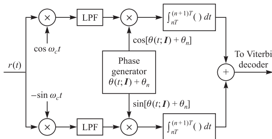
FIGURE 4.9-4 Computation of metric increments v_n(\mathbf{I}; \theta_n) .
