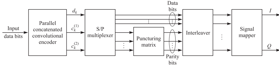
FIGURE 8.12–14 Encoder for concatenation of a PCCC (turbo code) with TCM.
