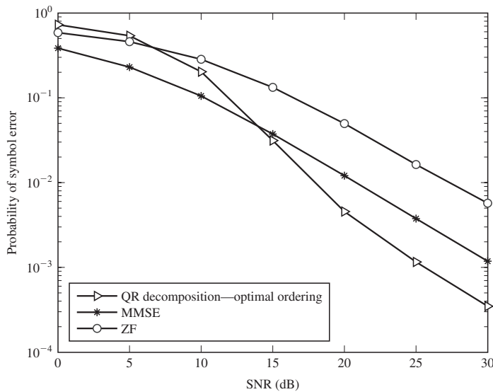
FIGURE 16.4-9 Comparison of the QR decomposition and the linear precoders with N_T = K = 6 .
