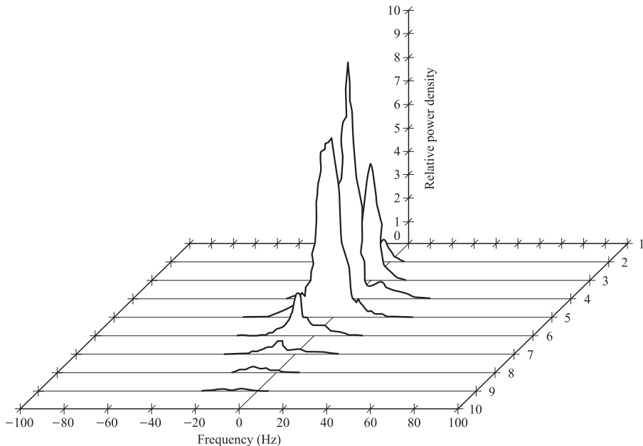
FIGURE 13.1-6 Scattering function of a medium-range tropospheric scatter channel. The taps delay increment is 0.1 \mu\text{s} .
