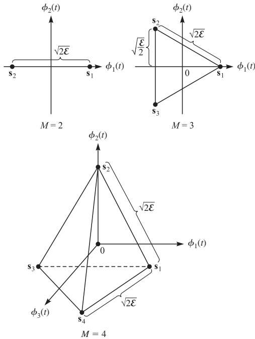
FIGURE 3.2-9 Signal space diagrams for M -ary simplex signals.
