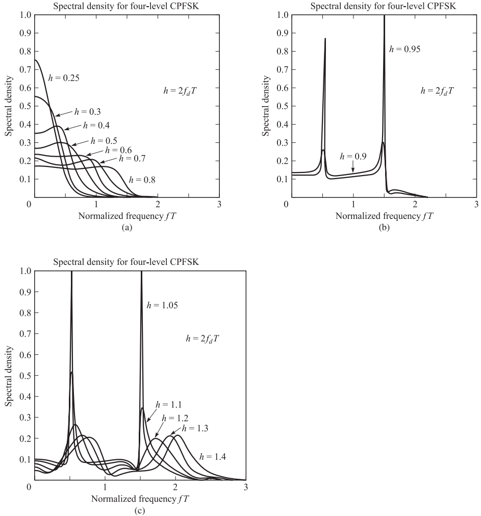
FIGURE 3.4-2 Power spectral density of quaternary CPFSK.
