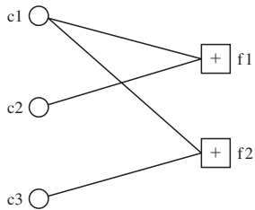
FIGURE 8.10-3 The Tanner graph for the (3, 1) repetition code.
