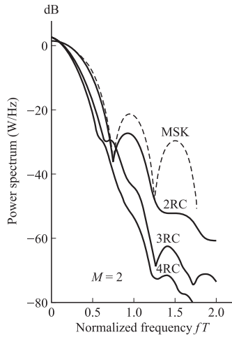
FIGURE 3.4-6 Power spectral density for binary CPM with h = \frac{1}{2} and different pulse shapes. [Source: Aulin et al. (1981); © IEEE.]
