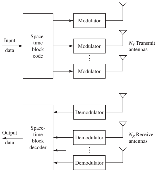
FIGURE 15.4-5 Space-time block coded MIMO system.
