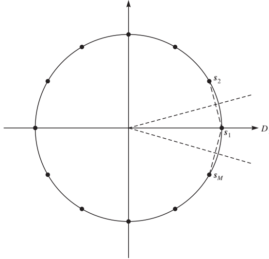
FIGURE 4.3-3 The constellation for PSK signaling.
