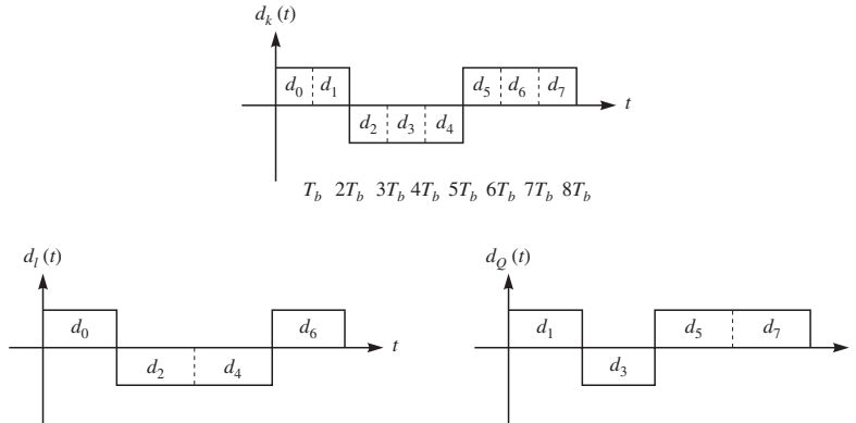
FIGURE 3.3-12 The in-phase and quadrature components for QPSK.
