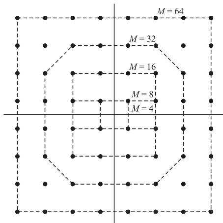
FIGURE 3.2-5 Several signal space diagrams for rectangular QAM.
