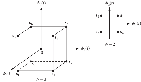
FIGURE 3.2-10 Signal space diagrams for signals generated from binary codes.
