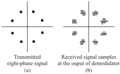
FIGURE 9.2-3 Two-dimensional digital “eye patterns.”
