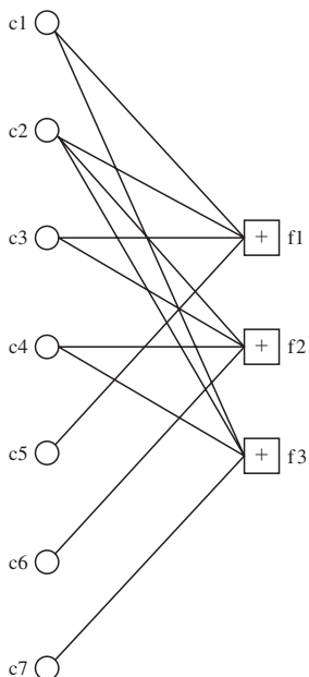
FIGURE 8.10-4 The Tanner graph for the (7, 4) Hamming code.
