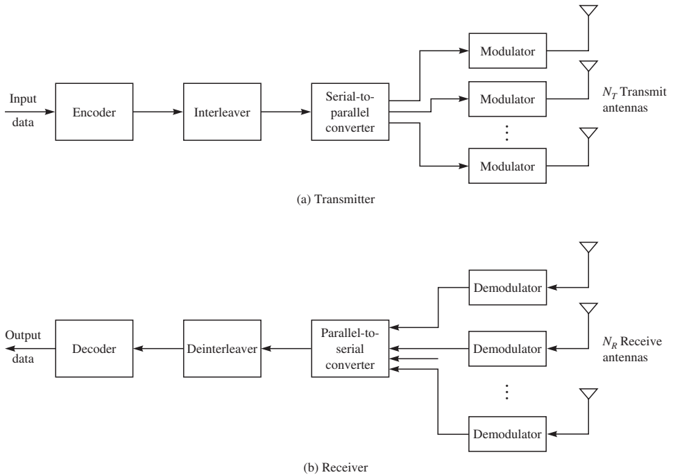
FIGURE 15.4-2 Bit-interleaved temporally coded MIMO system.
