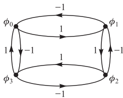
FIGURE 3.3-9 State trellis for binary CPFSK with h = \frac{1}{2} .
