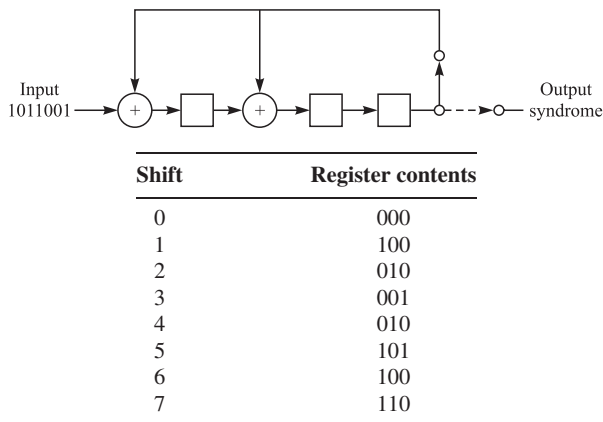
FIGURE 7.9-7 Syndrome computation for the (7, 4) cyclic code with generator polynomial g(X) = X^3 + X + 1 and received vector \mathbf{y} = (1001101) .
