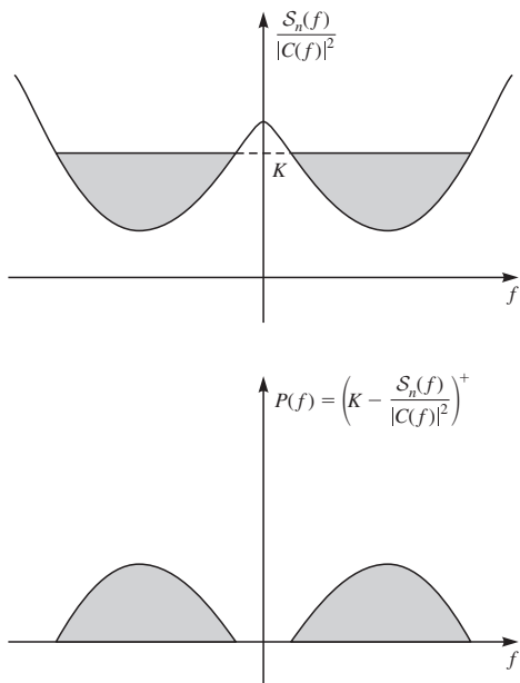
FIGURE 14.1-1 The water-filling interpretation of the channel capacity.
