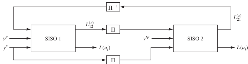
FIGURE 8.9–3 Block diagram of a turbo decoder.
