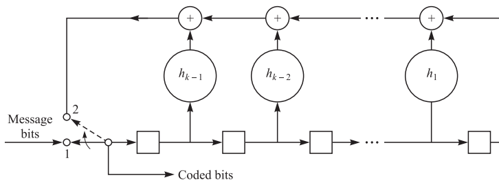
FIGURE 7.9-4 The encoder for an (n, k) cyclic code based on the parity polynomial h(X) .
