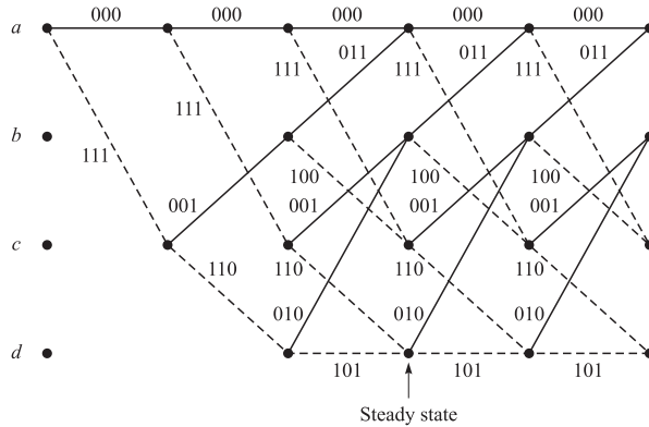
FIGURE 8.1-6 Trellis diagram for rate 1/3, K = 3 convolutional code.
