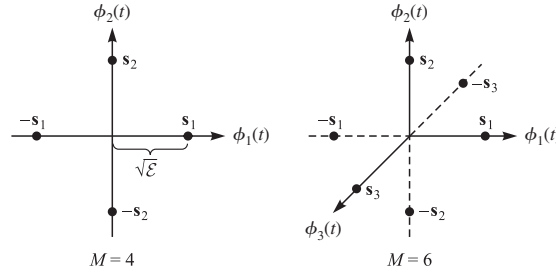
FIGURE 3.2-8 Signal space diagram for M = 4 and M = 6 biorthogonal signals.
