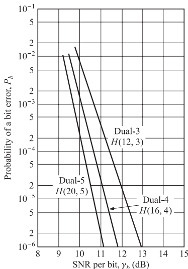
FIGURE 12.3-7 Performance of dual- k codes concatenated with Hadamard codes for a channel with worst-case partial-band interference.
