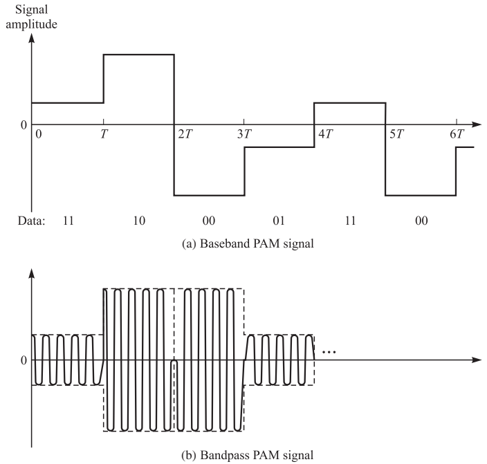
FIGURE 3.2-2 Example of (a) baseband and (b) carrier-modulated PAM signals.
