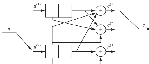
FIGURE 8.1-4 Double shift register implementation of the convolutional encoder shown in Figure 8.1-3.
