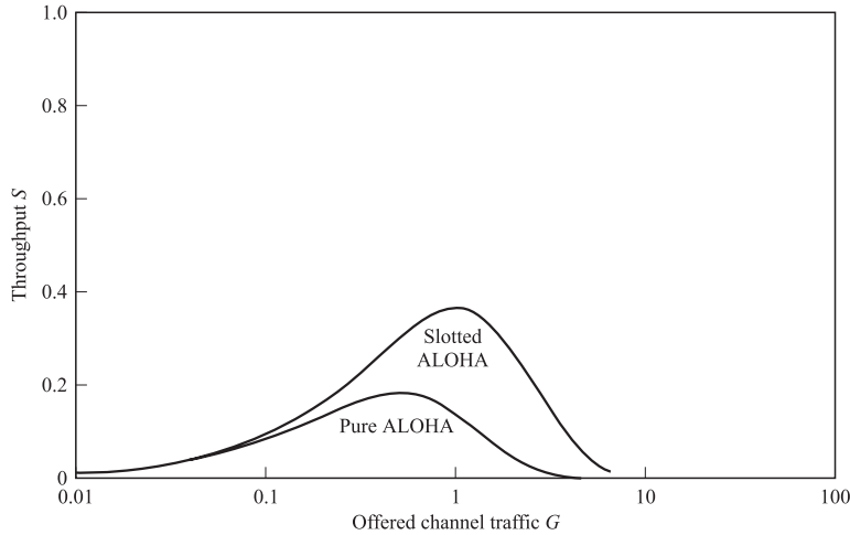
FIGURE 16.5-3 Throughput in ALOHA systems.
