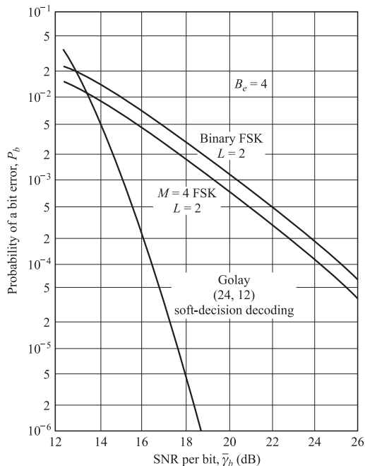
FIGURE 14.7-1 Example of performance obtained with conventional diversity versus coding for B_e = 4 .
