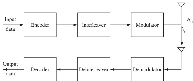
FIGURE 15.4–1 Temporally coded SISO system.
