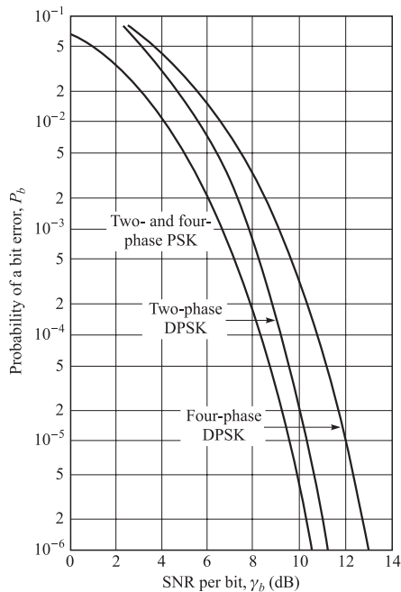
FIGURE 4.5-6 Probability of bit error for binary and four-phase PSK and DPSK.
