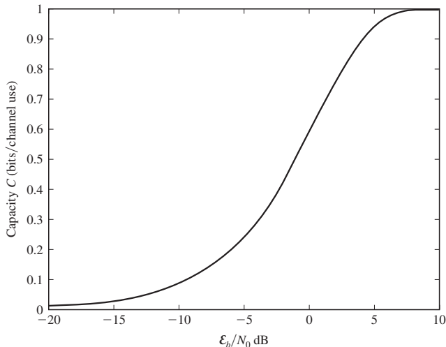
FIGURE 6.5-5 The capacity plot versus SNR per bit.
