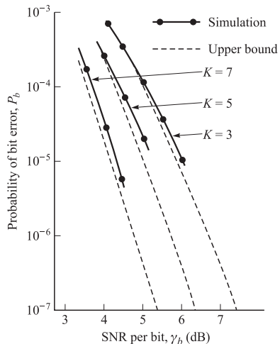
FIGURE 8.6-2 Bit error probability for rate 1/2 Viterbi decoding with eight-level quantized inputs to the decoder and 32-bit path memory. [From Heller and Jacobs (1971). © 1971 IEEE.]
