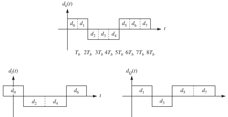
FIGURE 3.3-14 The in-phase and quadrature components for OQPSK signaling.
