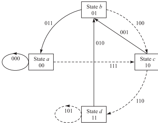
FIGURE 8.1-7 State diagram for rate 1/3, K = 3 convolutional code.
