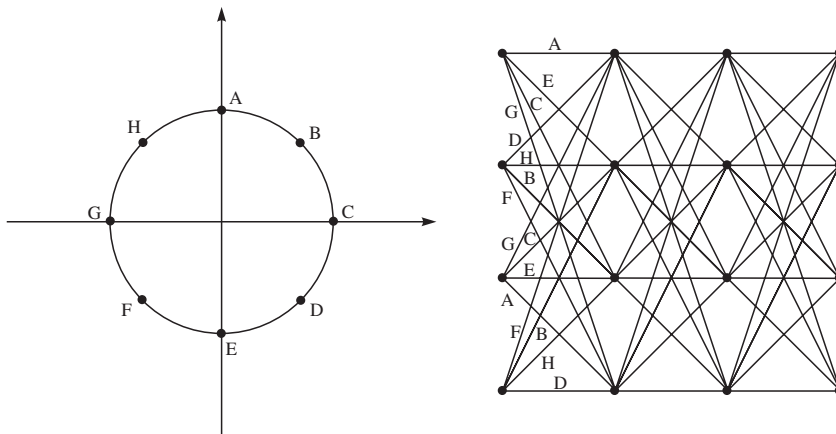
FIGURE 14.5–2 The improved TCM scheme.
